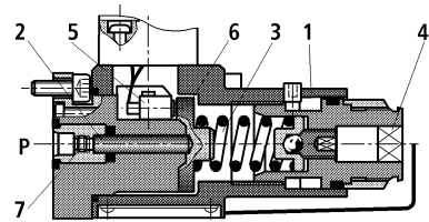
型号HED 8 OH1X/...K14 A / AS ...
