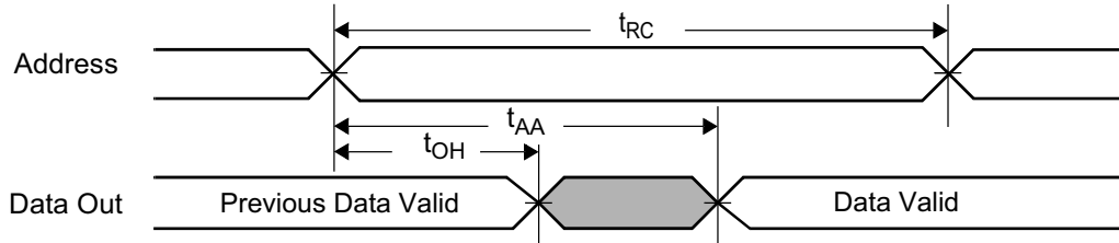
READ CYCLE (1) (Address controlled, CS#=OE#=V IL , ZZ#=WE#=V IH , UB# or/and LB#=V IL )
