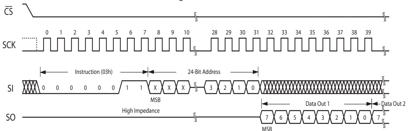
Figure 2.5 READ
