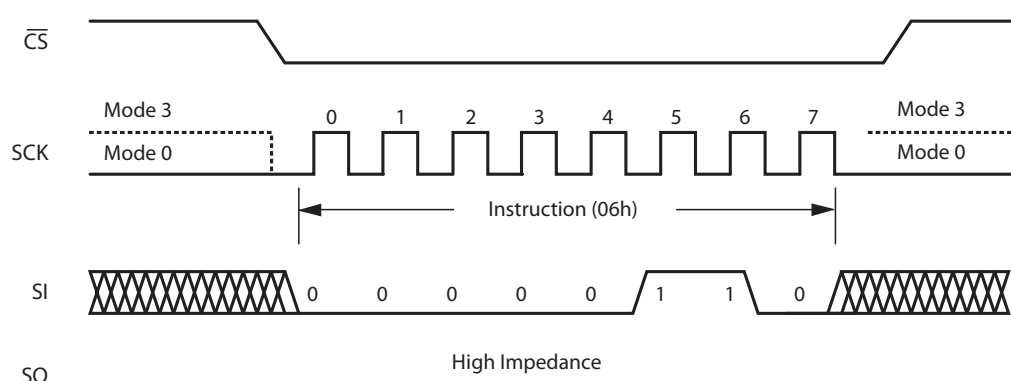
Figure 2.2 WREN
