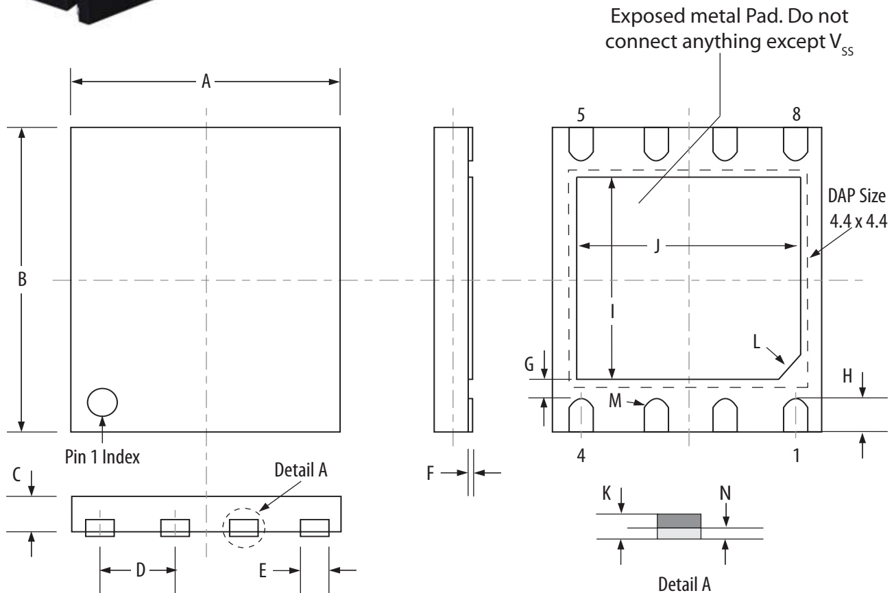
Figure 6.1 DFN Package
