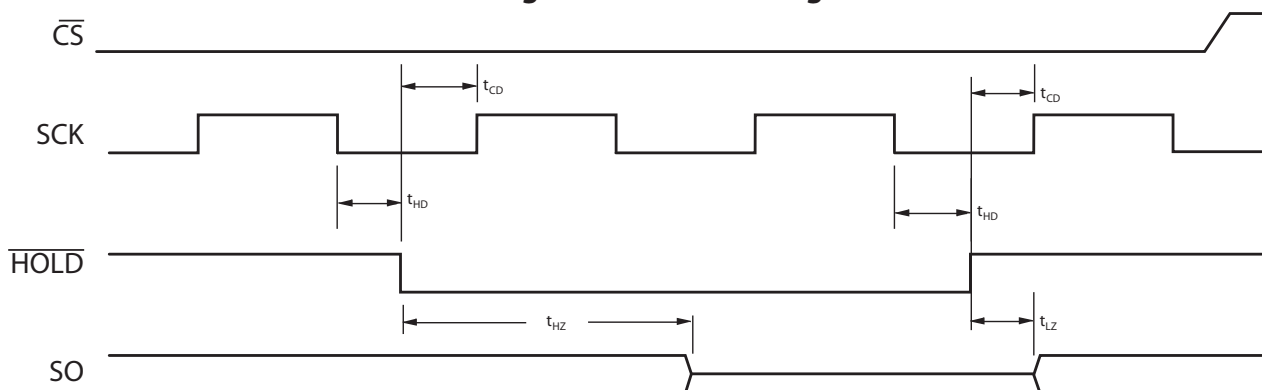
Figure 4.5 HOLD Timing
