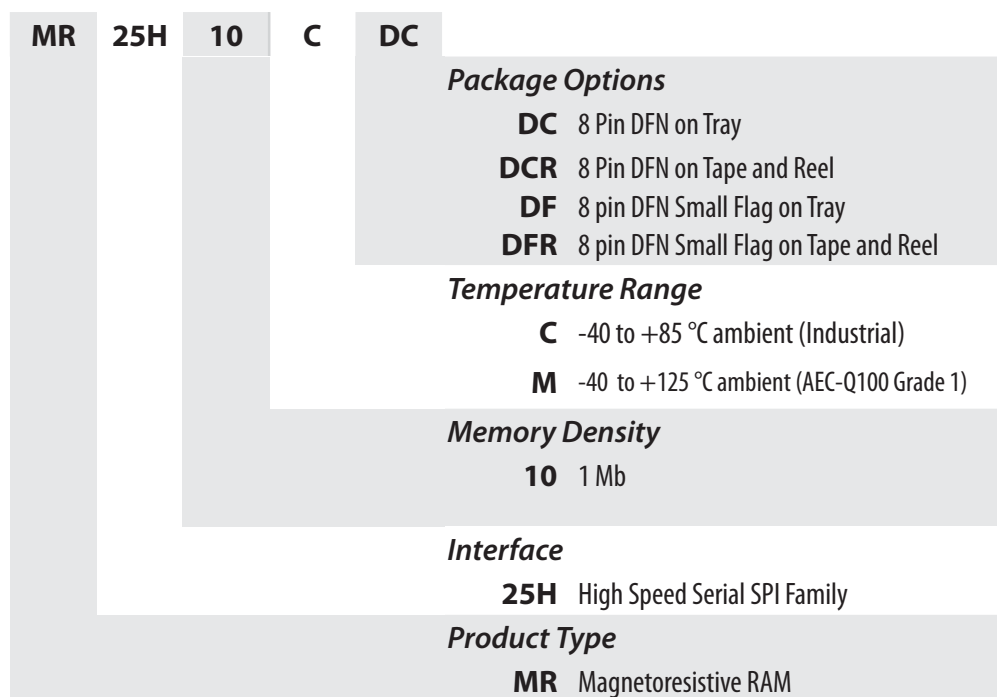
Figure 5.1 Part Numbering System
