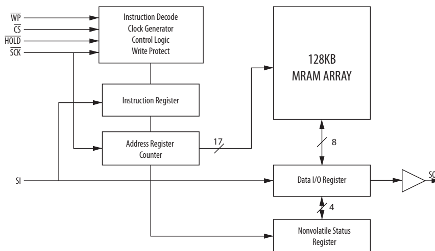
Figure 1.1 Block Diagram
