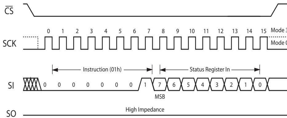
Figure 2.4 WRSR
