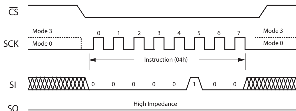
Figure 2.3 WRDI
