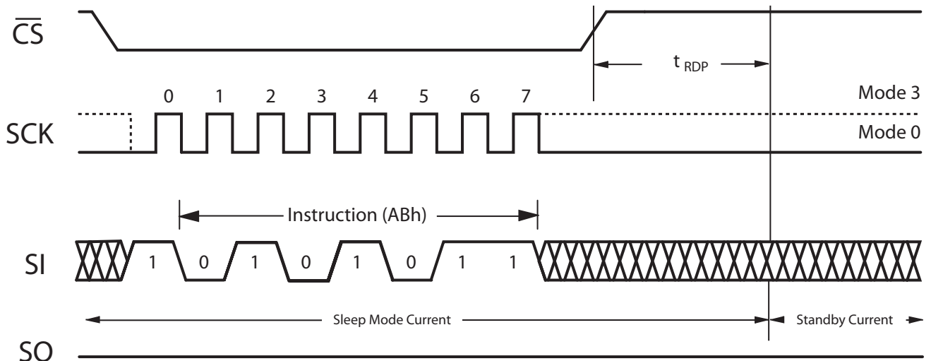
Figure 2.8 WAKE
