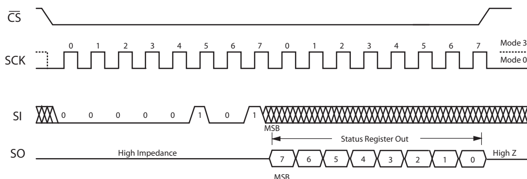
Figure 2.1 RDSR
