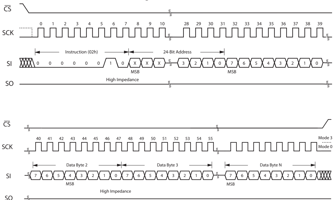
Figure 2.6 WRITE
