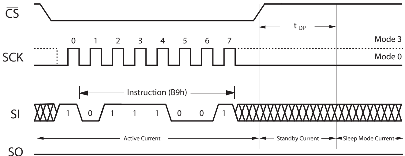
Figure 2.7 SLEEP
