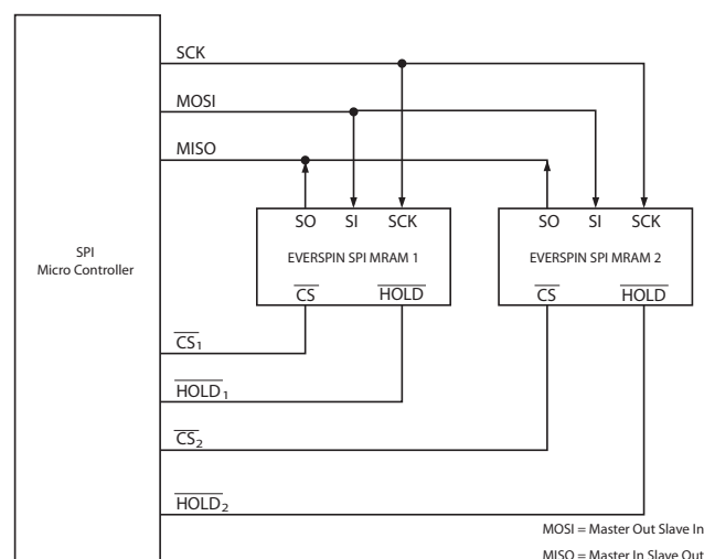
Figure 1.2 System Configuration
