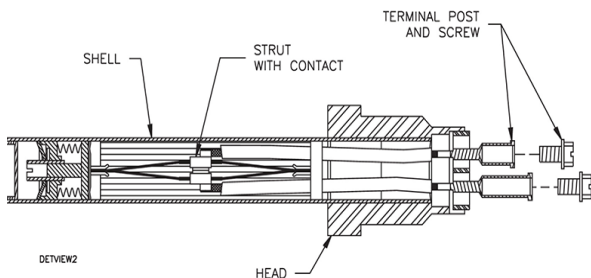
Figure 1. Fire/Overheat Detector
