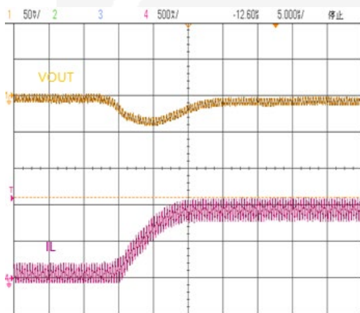
Transient ripple at 0.1A~1A
