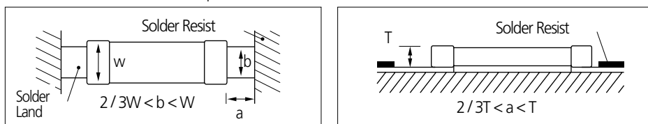
Recommendation of solder Land Shape and Size
