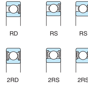
Extremely light contact sealed Contact sealed
