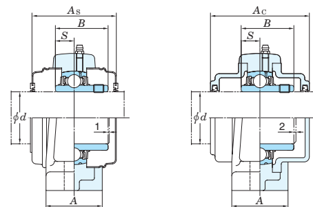
Pressed steel covers
