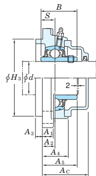
Cast iron cover
