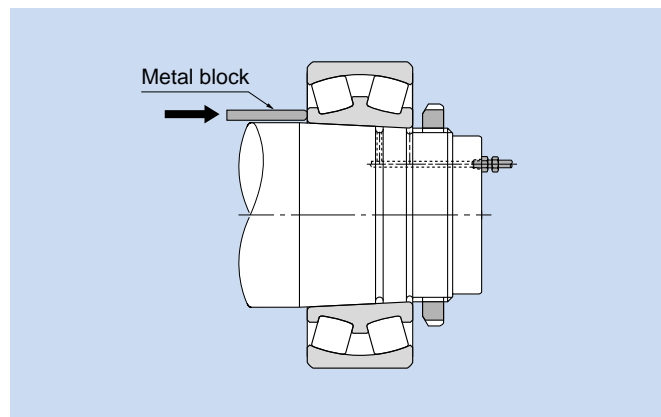
Fig. 15.23 Disassembly using high pressure oil (hydraulic)
