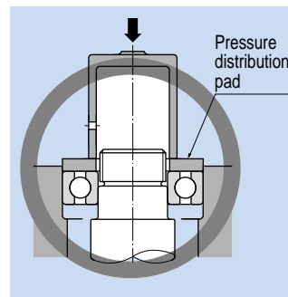
Fig. 15.4 Fitting sleeve pressure against inner /outer ring simultaneously pressure against inner ring
