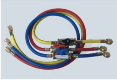
CCL-36-1/2"-20 UNF-1/4" SAE
