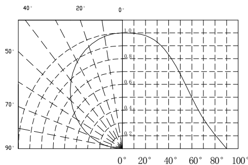
Diagram characteristics of radiation
