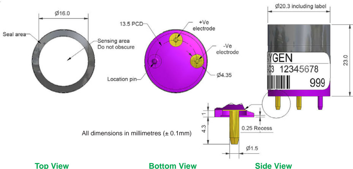
Figure 1 O2-C3 Schematic Diagram
