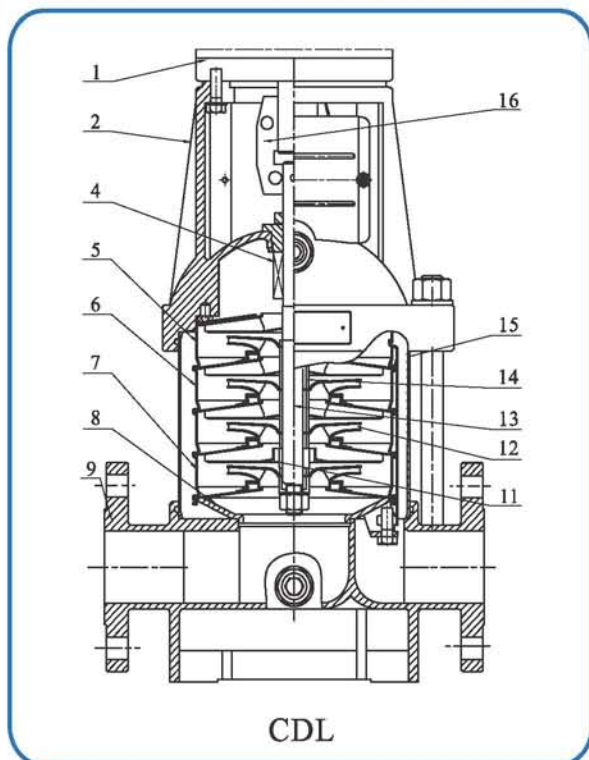
截面图 CDL, CDLF8, 10, 12, 15, 16, 20
